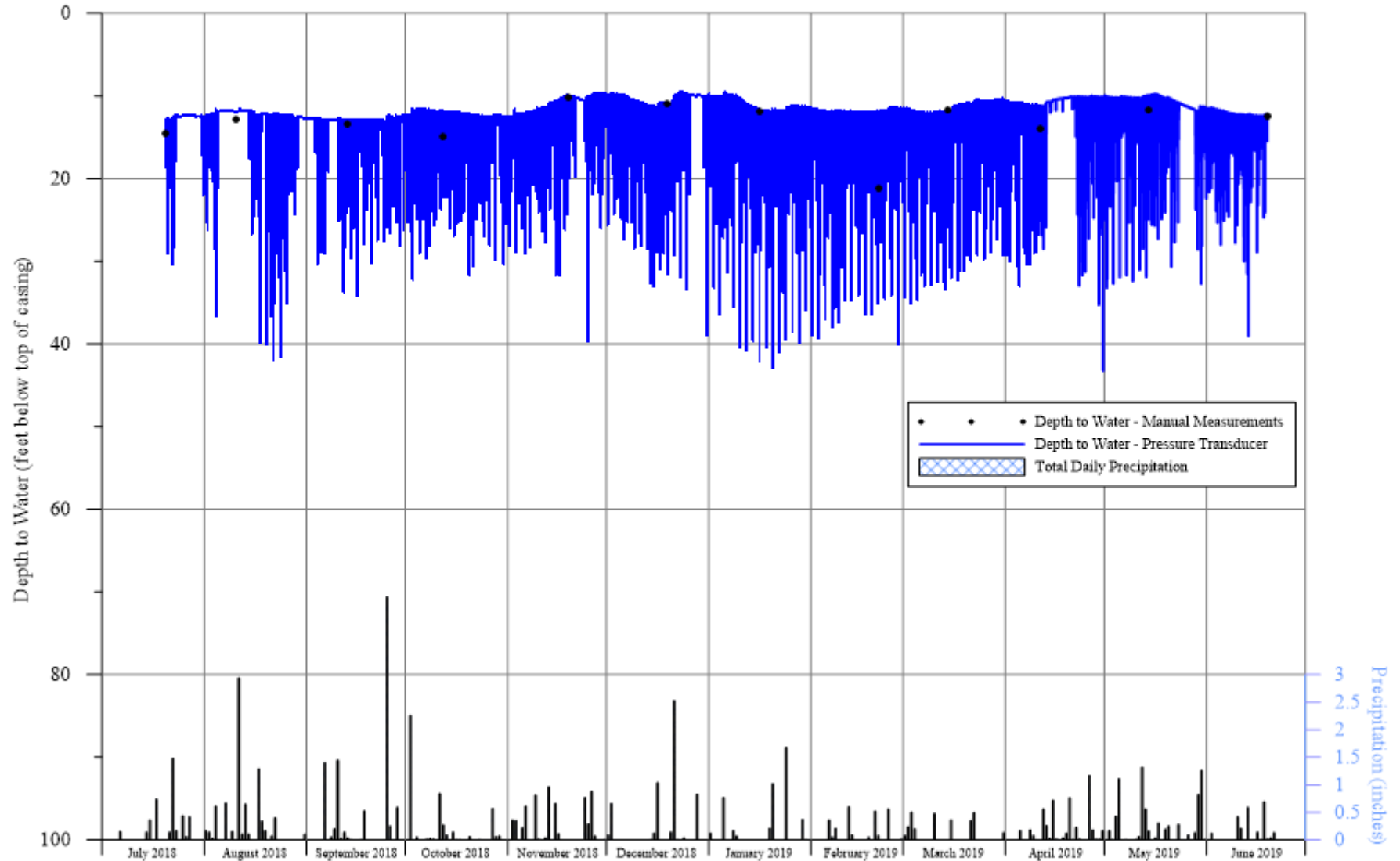
Well Monitoring Program Hydrograph of Water-Level Measurements Collected from Well A
